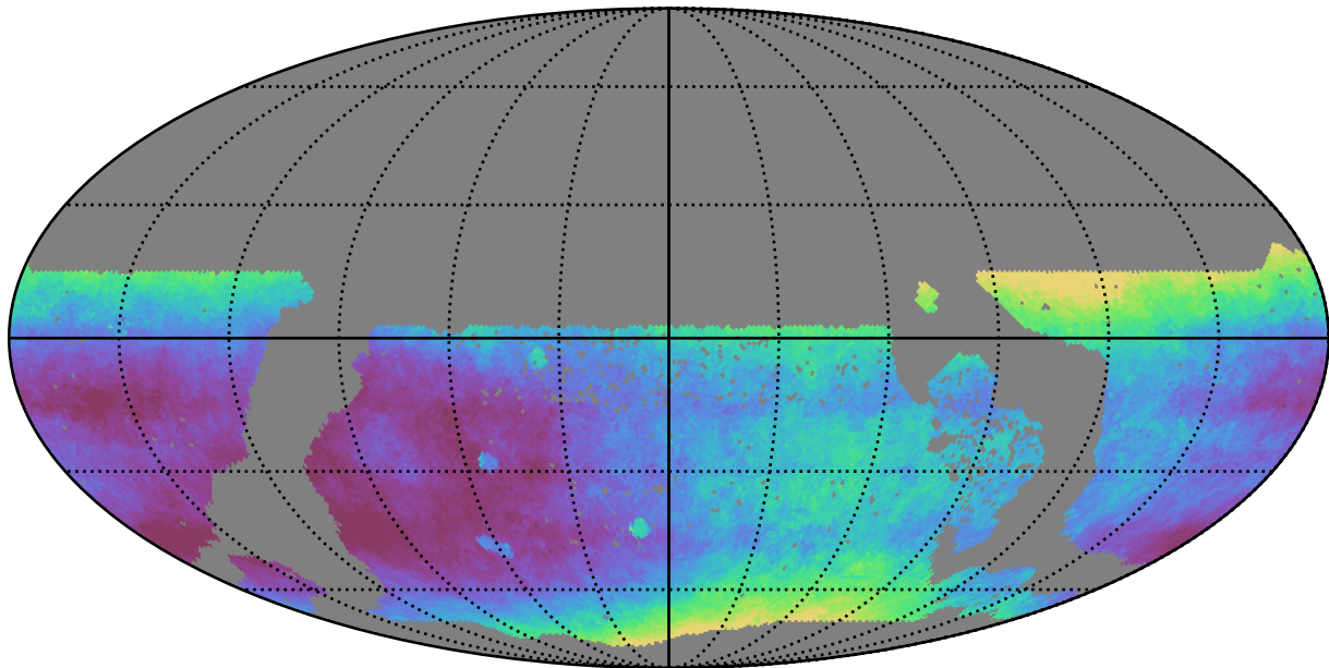
too_elab_r64_d2_giz_v3.4_10yrs WFD all bands: Median seeingEff
