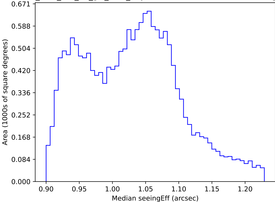
too_elab_r64_d2_giz_v3.4_10yrs WFD all bands: Median seeingEff
