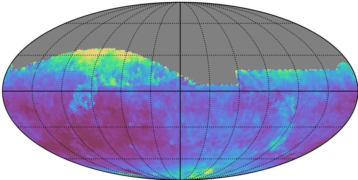
too_elab_r64_d2_giz_v3.4_10yrs All sky z band: Median seeingEff
