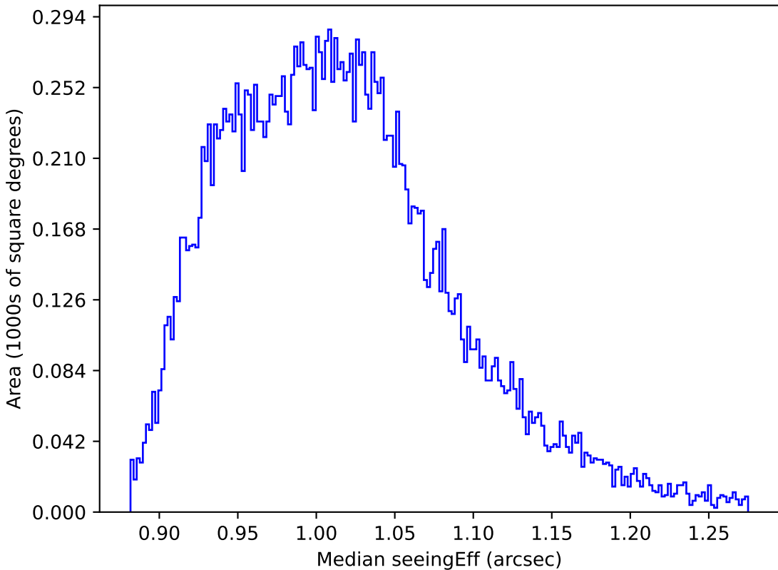
too_elab_r64_d2_giz_v3.4_10yrs All sky y band: Median seeingEff
