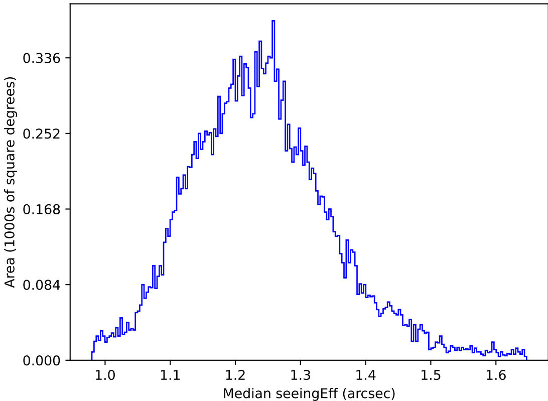
too_elab_r64_d2_giz_v3.4_10yrs All sky u band: Median seeingEff
