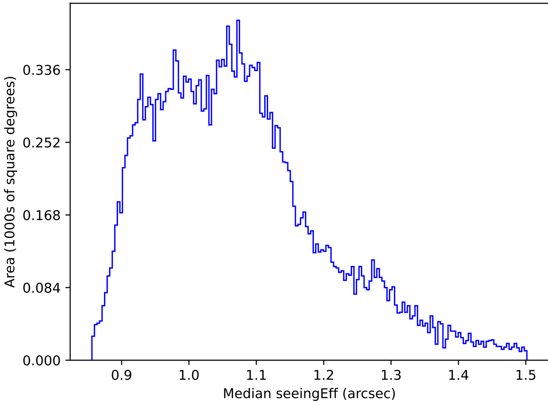
too_elab_r64_d2_giz_v3.4_10yrs All sky r band: Median seeingEff
