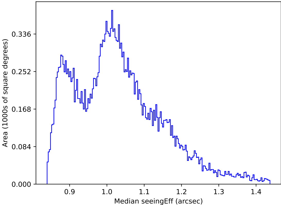
too_elab_r64_d2_giz_v3.4_10yrs All sky i band: Median seeingEff
