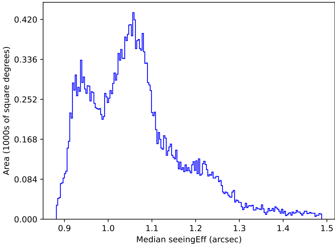
too_elab_r64_d2_giz_v3.4_10yrs All sky all bands: Median seeingEff
