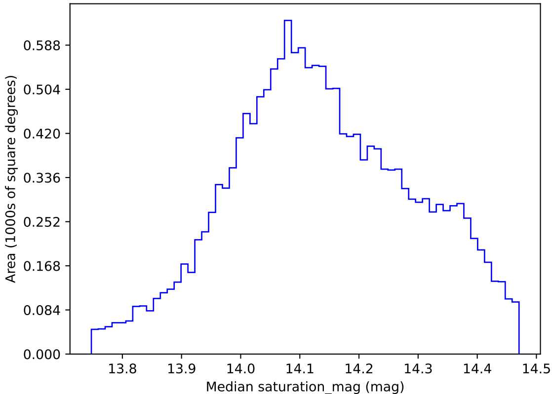
too_elab_r64_d2_giz_v3.4_10yrs WFD z band: Median saturation_mag
