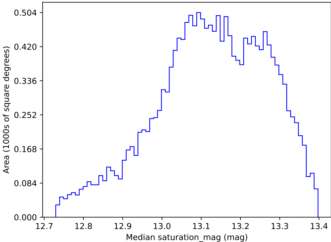
too_elab_r64_d2_giz_v3.4_10yrs WFD y band: Median saturation_mag
