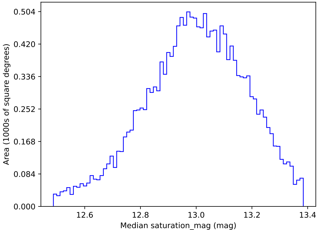
too_elab_r64_d2_giz_v3.4_10yrs WFD u band: Median saturation_mag
