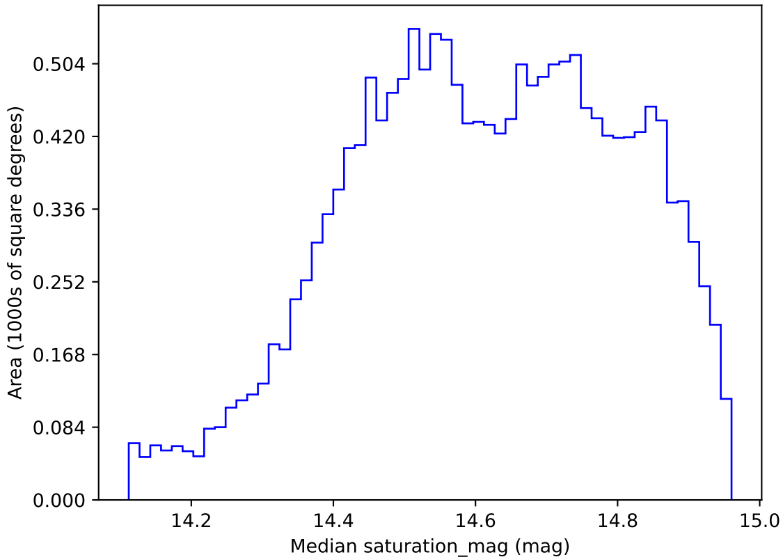
too_elab_r64_d2_giz_v3.4_10yrs WFD r band: Median saturation_mag
