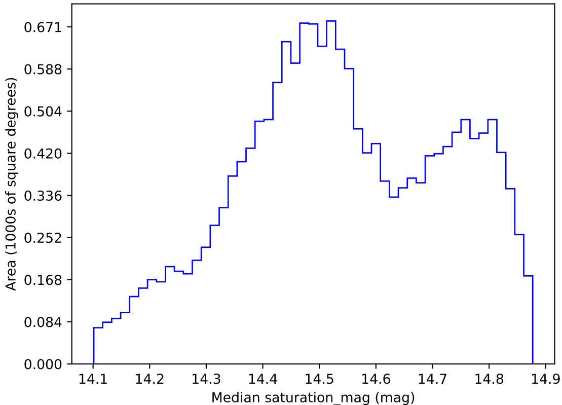
too_elab_r64_d2_giz_v3.4_10yrs WFD i band: Median saturation_mag
