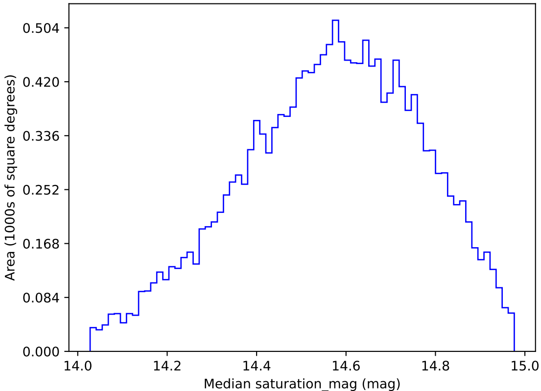
too_elab_r64_d2_giz_v3.4_10yrs WFD g band: Median saturation_mag
