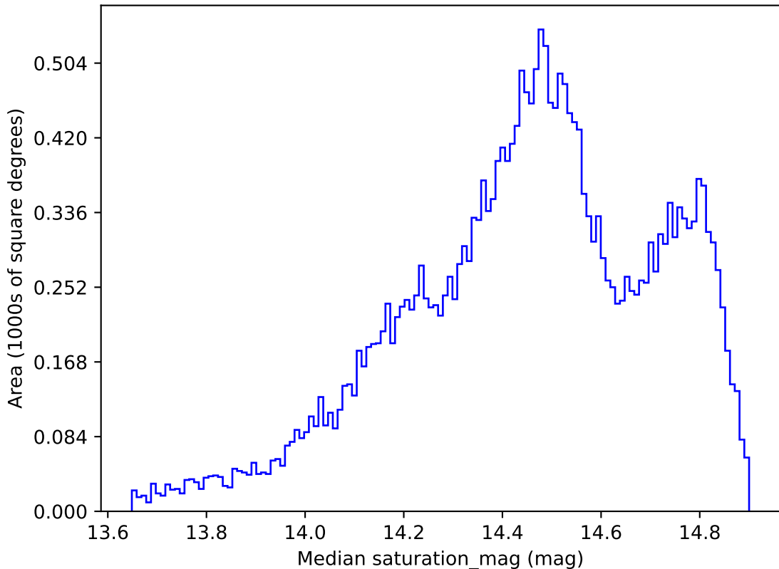
too_elab_r64_d2_giz_v3.4_10yrs All sky i band: Median saturation_mag
