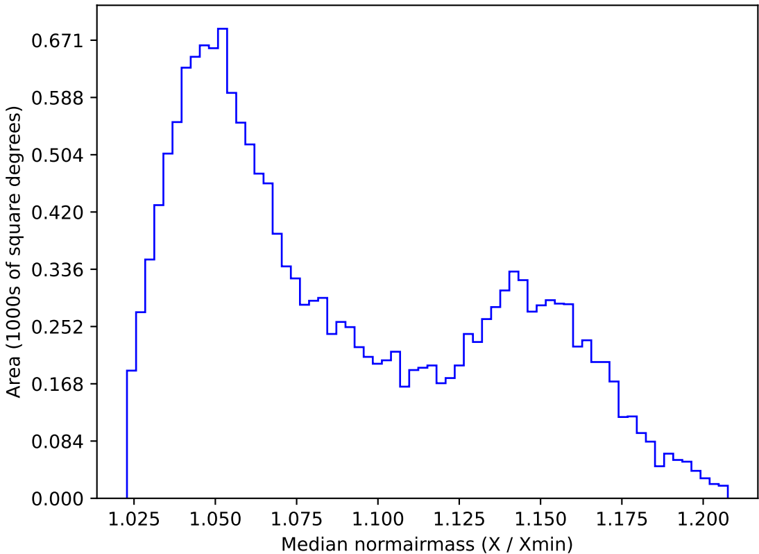
too_elab_r64_d2_giz_v3.4_10yrs WFD z band: Median normairmass
