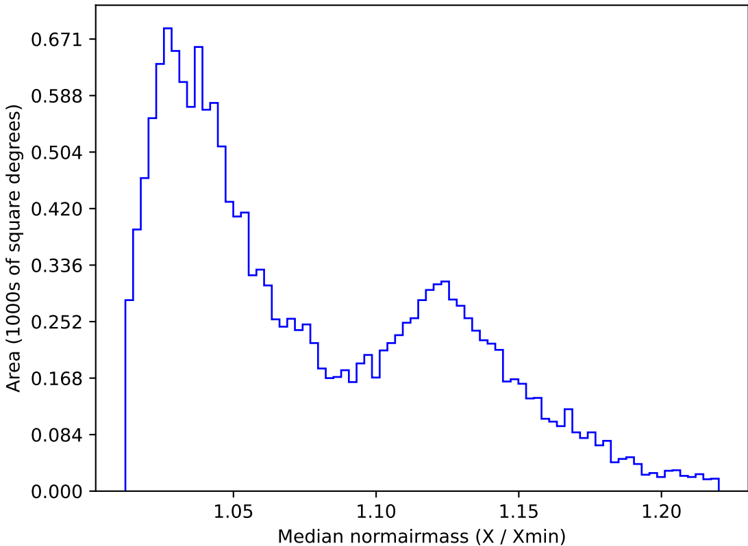
too_elab_r64_d2_giz_v3.4_10yrs WFD u band: Median normairmass
