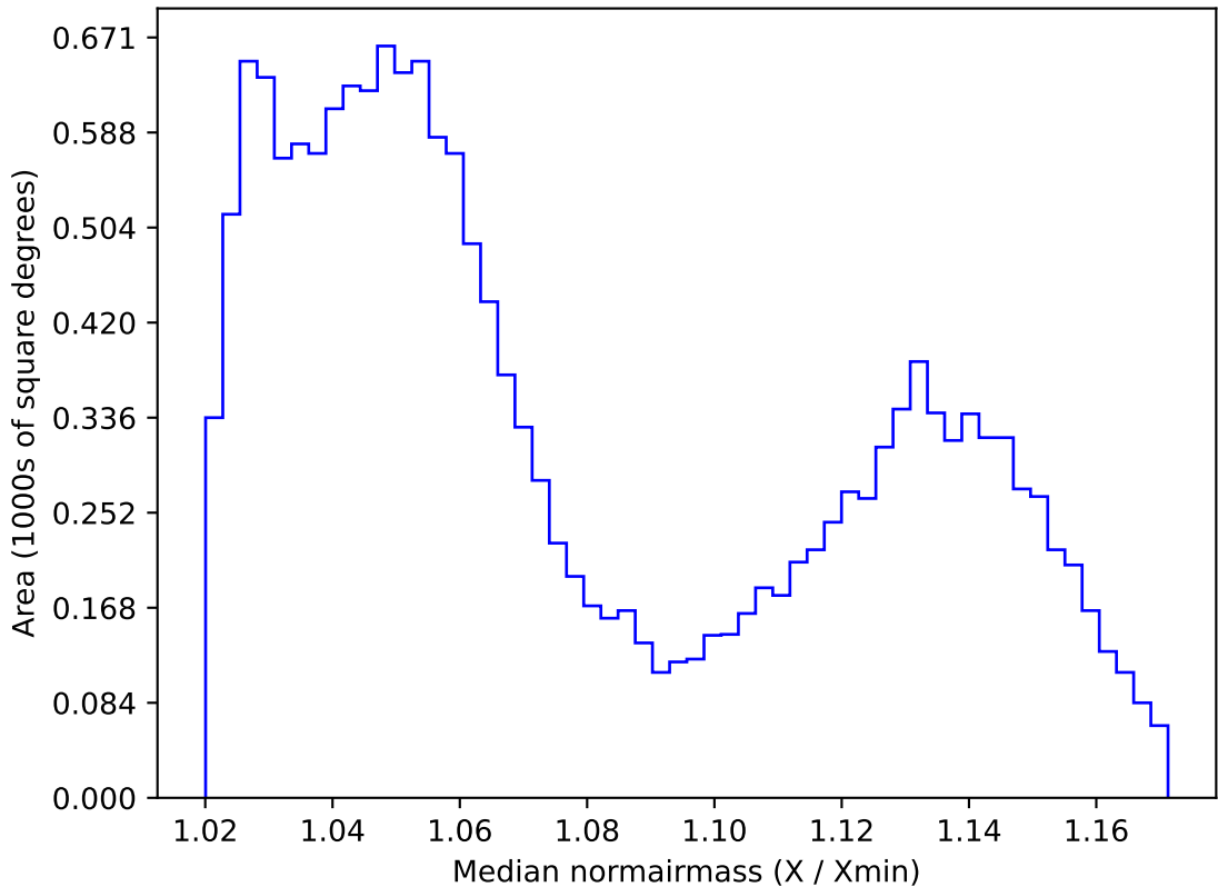
too_elab_r64_d2_giz_v3.4_10yrs WFD i band: Median normairmass
