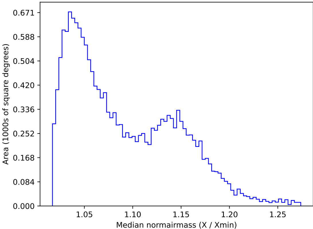
too_elab_r64_d2_giz_v3.4_10yrs WFD g band: Median normairmass
