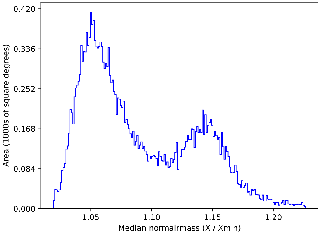
too_elab_r64_d2_giz_v3.4_10yrs All sky y band: Median normairmass
