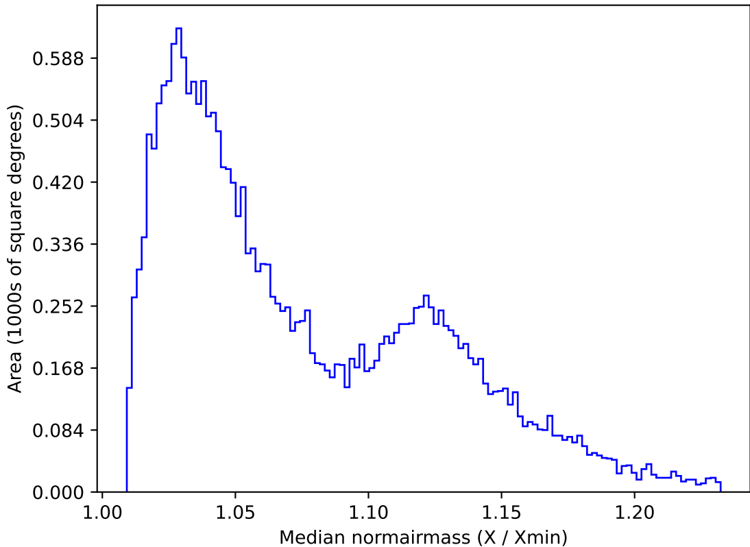
too_elab_r64_d2_giz_v3.4_10yrs All sky u band: Median normairmass
