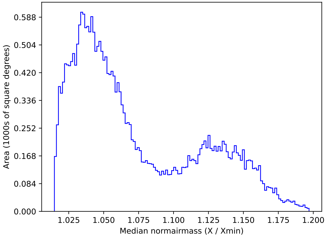
too_elab_r64_d2_giz_v3.4_10yrs All sky r band: Median normairmass
