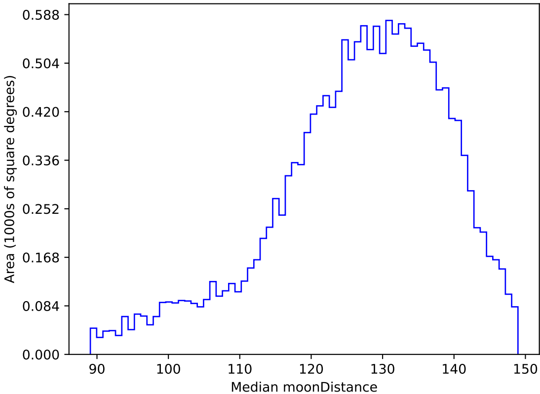
too_elab_r64_d2_giz_v3.4_10yrs WFD u band: Median moonDistance
