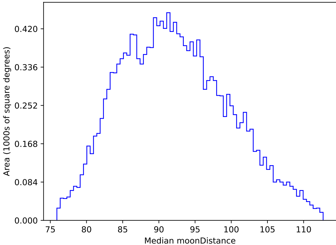
too_elab_r64_d2_giz_v3.4_10yrs WFD i band: Median moonDistance
