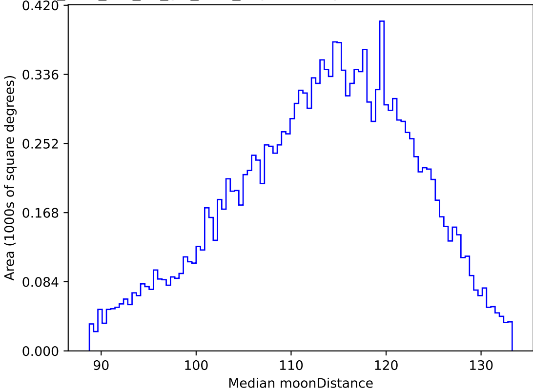
too_elab_r64_d2_giz_v3.4_10yrs WFD g band: Median moonDistance
