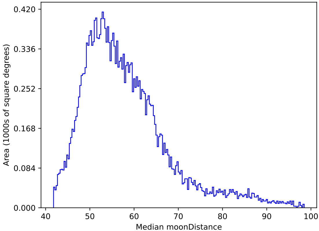
too_elab_r64_d2_giz_v3.4_10yrs All sky y band: Median moonDistance
