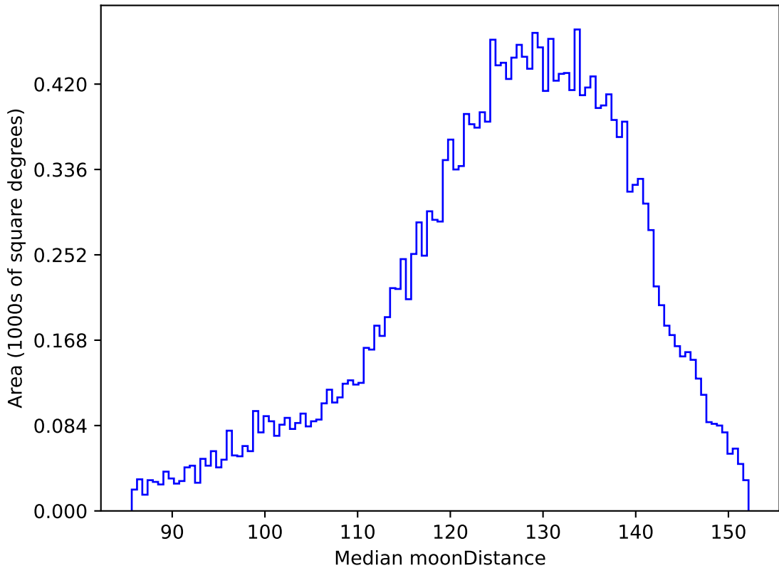
too_elab_r64_d2_giz_v3.4_10yrs All sky u band: Median moonDistance
