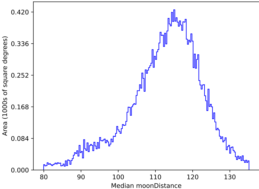
too_elab_r64_d2_giz_v3.4_10yrs All sky r band: Median moonDistance
