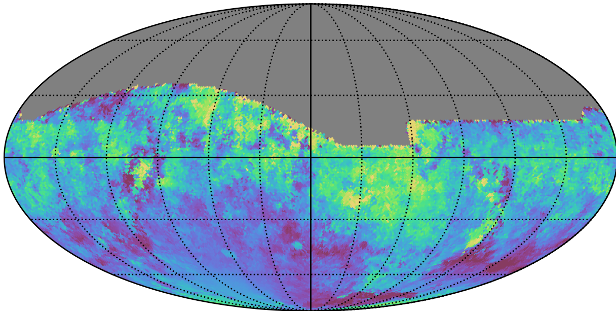
too_elab_r64_d2_giz_v3.4_10yrs All sky i band: Median moonDistance
