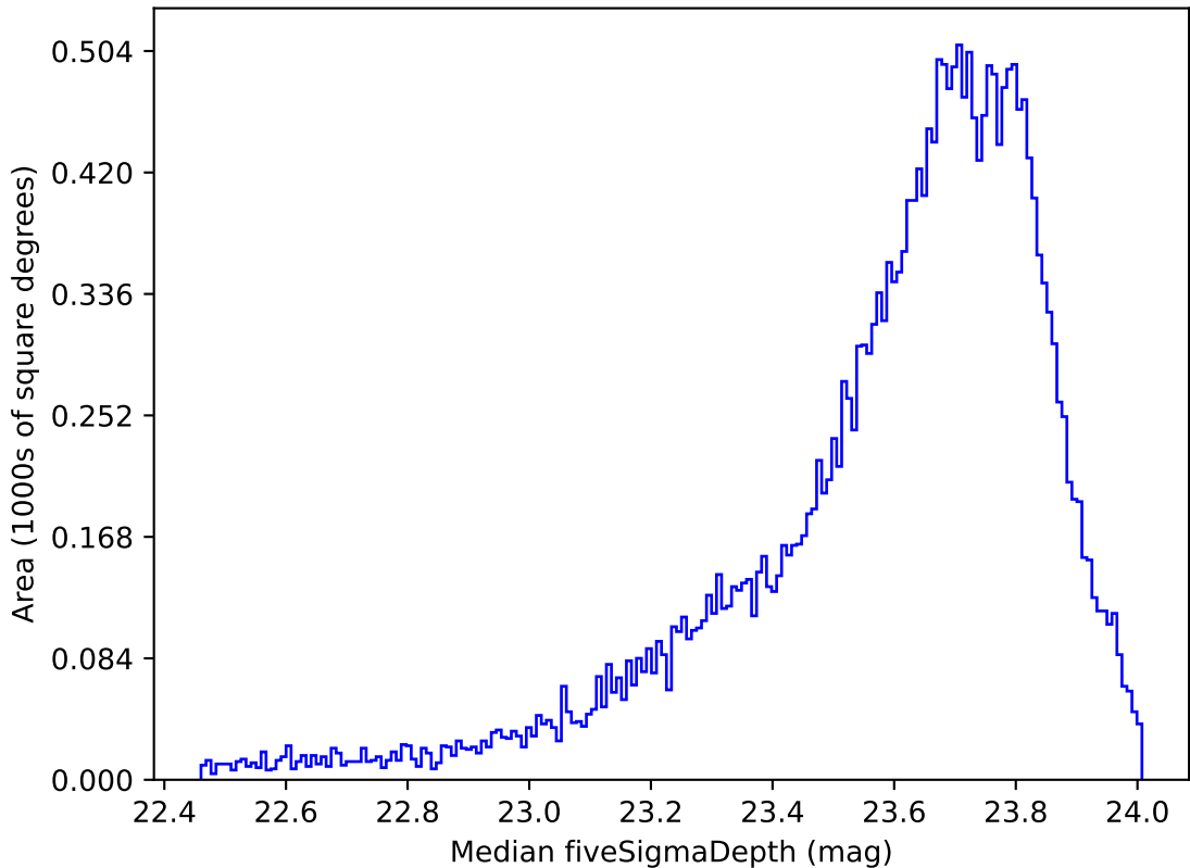
too_elab_r64_d2_giz_v3.4_10yrs Yr 1 i band: Median fiveSigmaDepth
