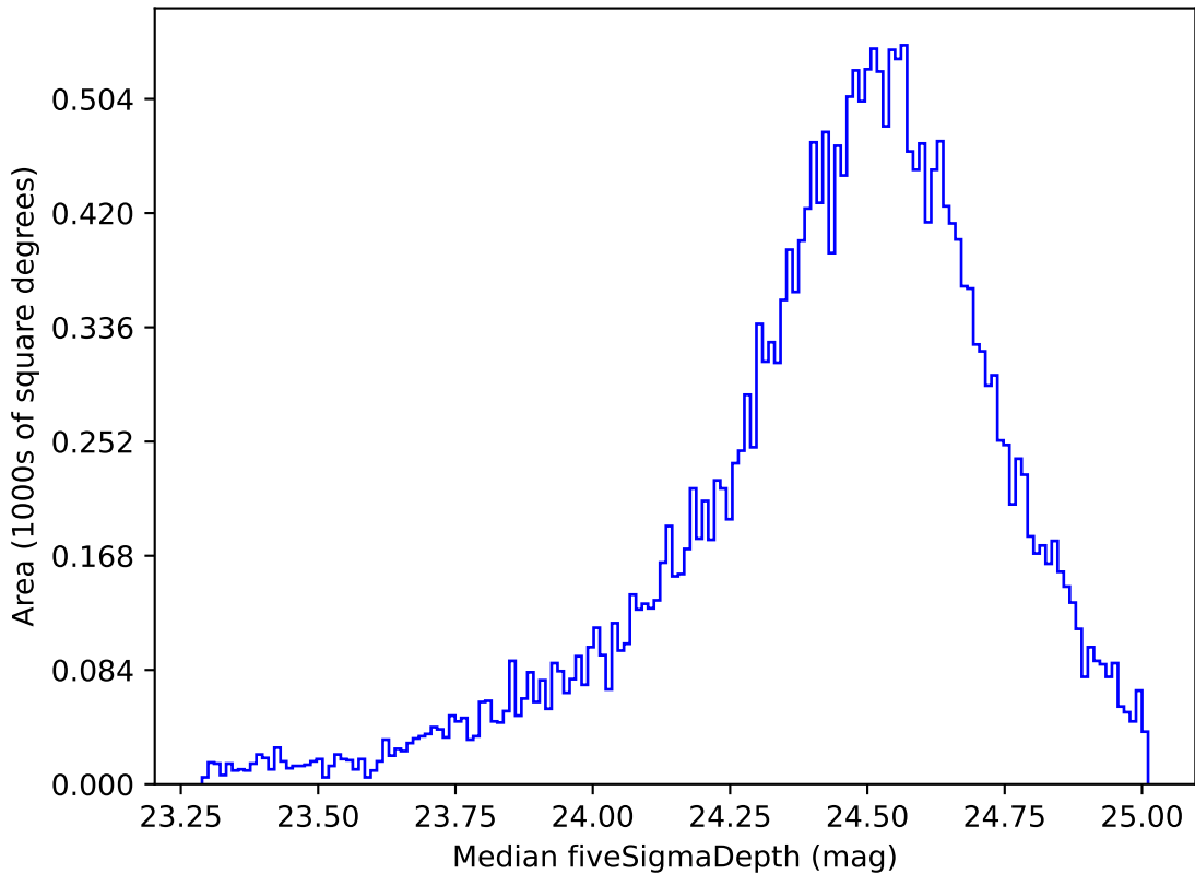
too_elab_r64_d2_giz_v3.4_10yrs Yr 1 g band: Median fiveSigmaDepth
