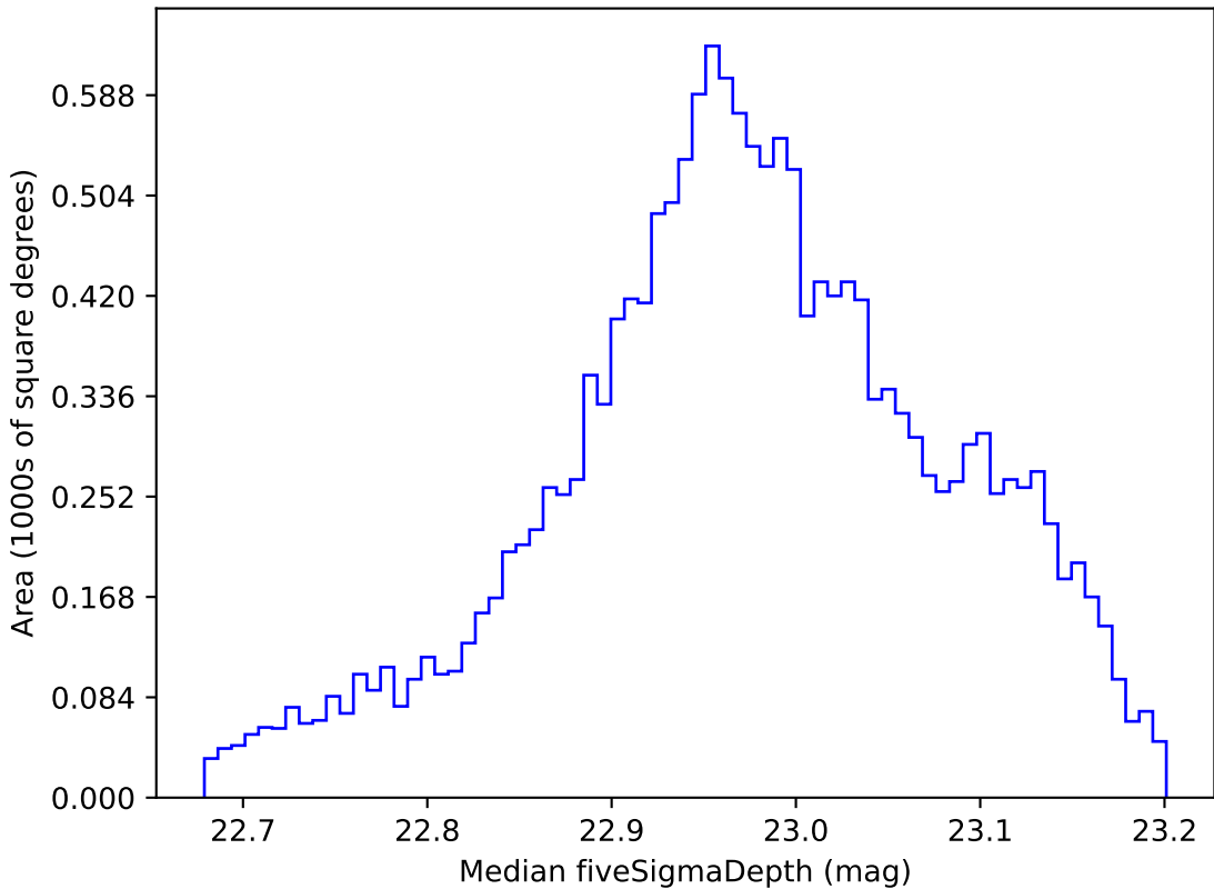
too_elab_r64_d2_giz_v3.4_10yrs WFD z band: Median fiveSigmaDepth
