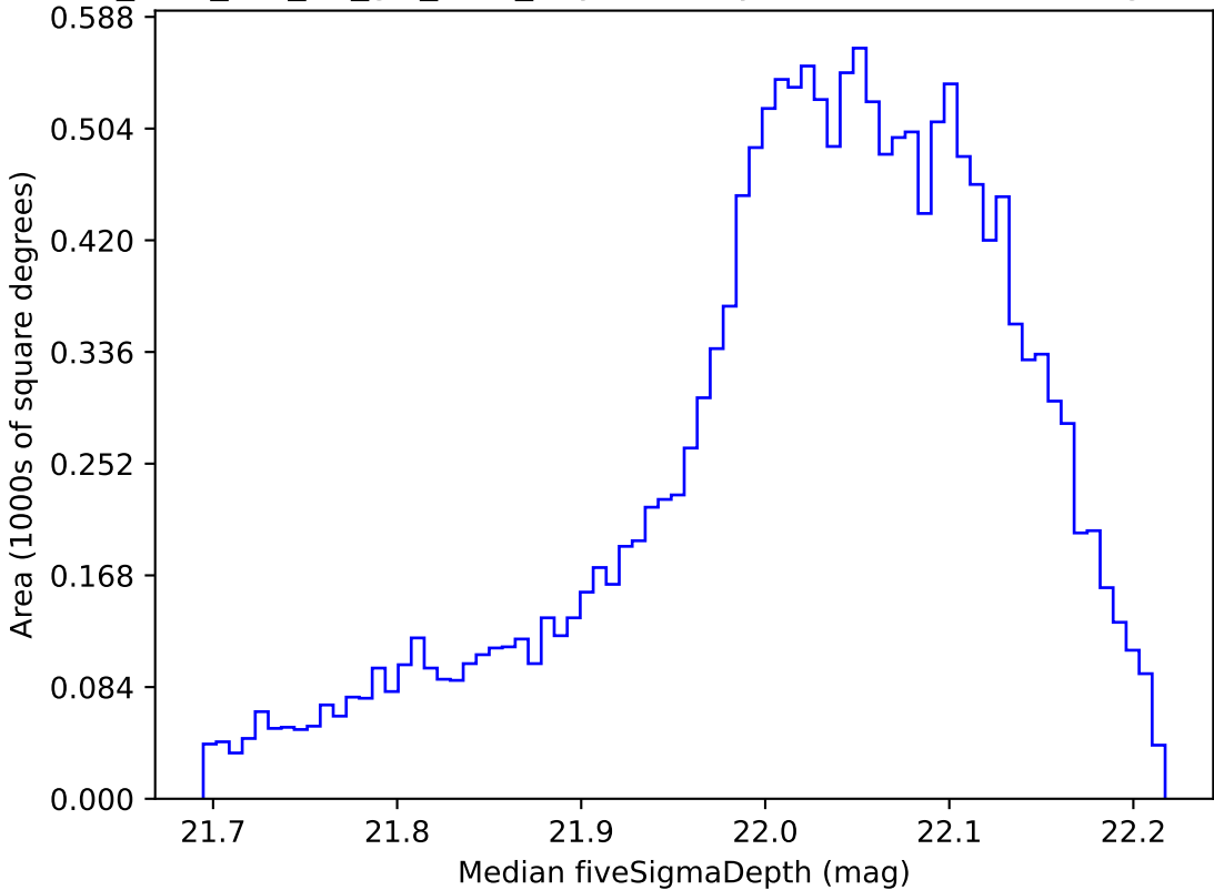
too_elab_r64_d2_giz_v3.4_10yrs WFD y band: Median fiveSigmaDepth
