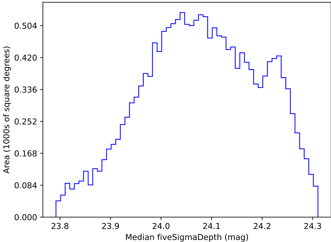
too_elab_r64_d2_giz_v3.4_10yrs WFD r band: Median fiveSigmaDepth
