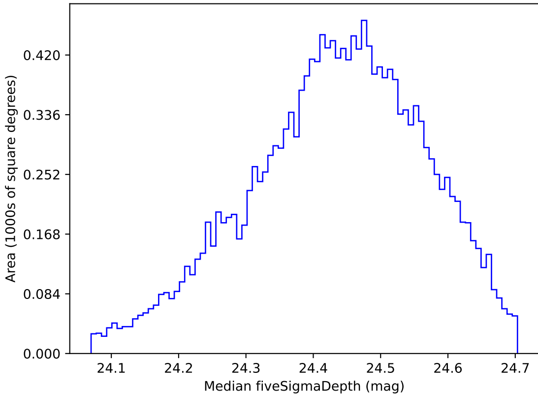
too_elab_r64_d2_giz_v3.4_10yrs WFD g band: Median fiveSigmaDepth
