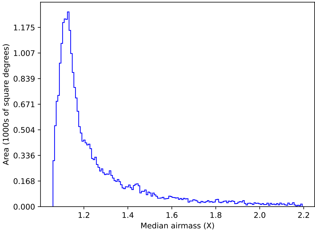
too_elab_r64_d2_giz_v3.4_10yrs Yr 1 z band: Median airmass
