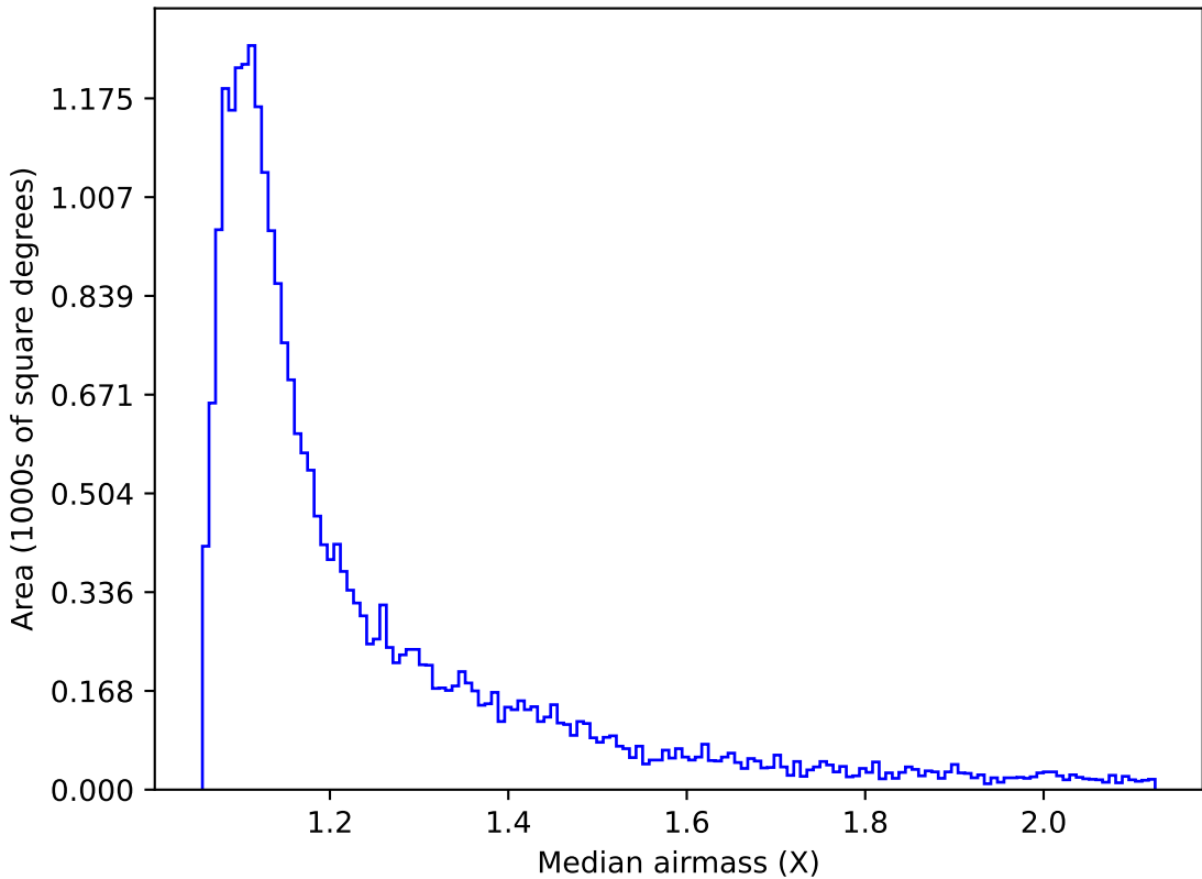
too_elab_r64_d2_giz_v3.4_10yrs Yr 1 r band: Median airmass
