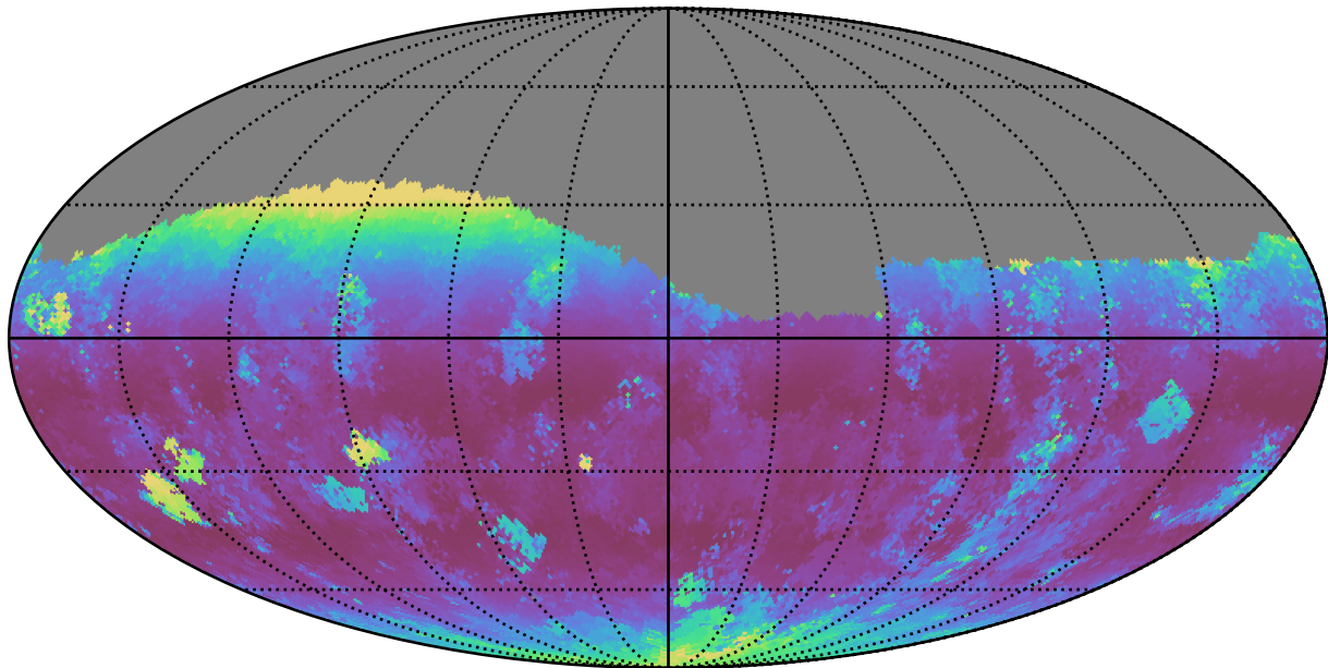
too_elab_r64_d2_giz_v3.4_10yrs Yr 1 g band: Median airmass
