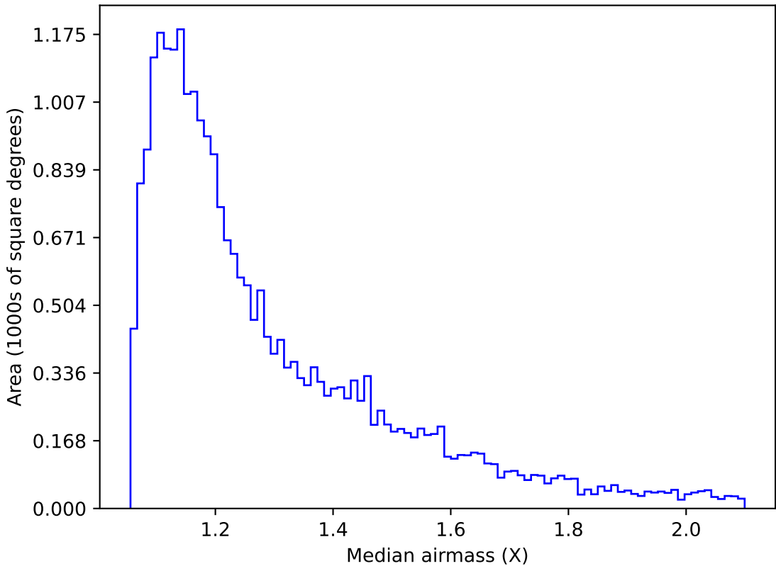
too_elab_r64_d2_giz_v3.4_10yrs Yr 1 g band: Median airmass
