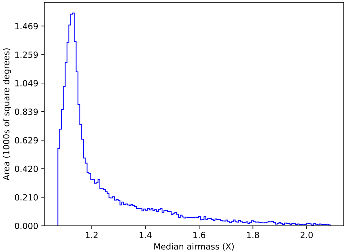
too_elab_r64_d2_giz_v3.4_10yrs Yr 1 all bands: Median airmass
