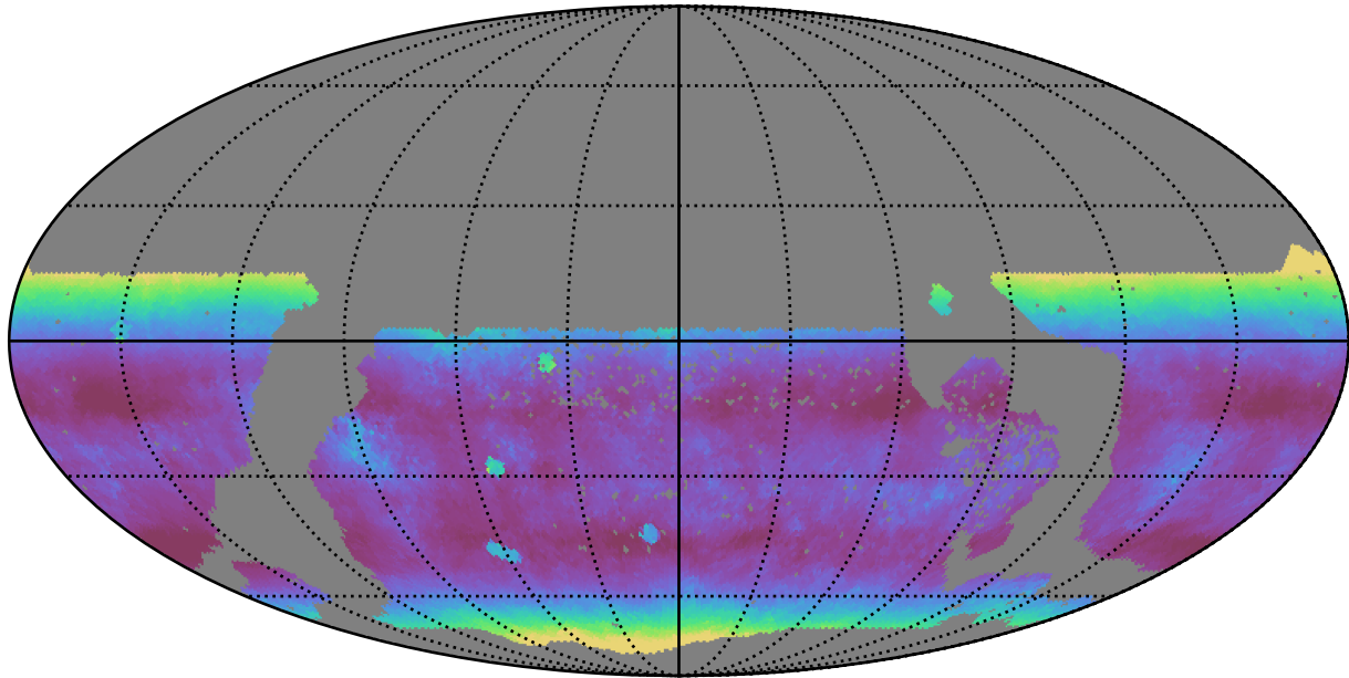
too_elab_r64_d2_giz_v3.4_10yrs WFD z band: Median airmass
