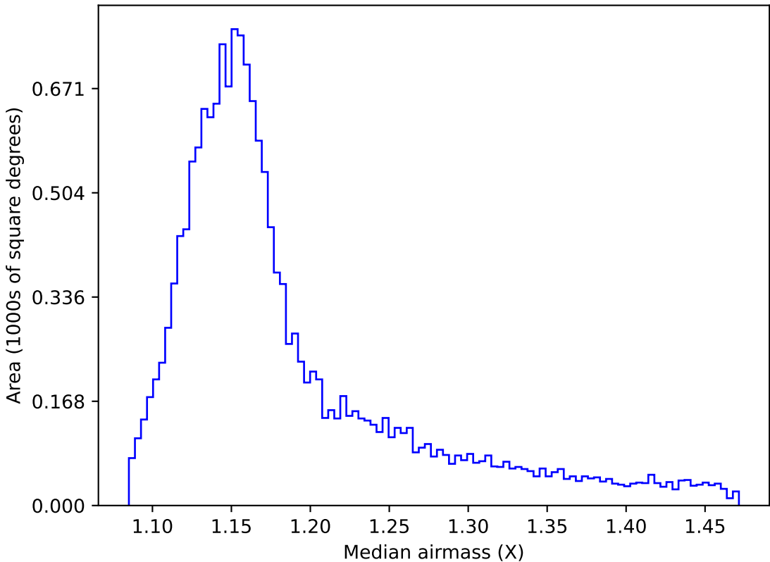
too_elab_r64_d2_giz_v3.4_10yrs WFD z band: Median airmass
