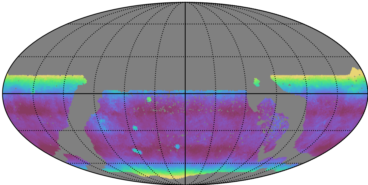
too_elab_r64_d2_giz_v3.4_10yrs WFD y band: Median airmass
