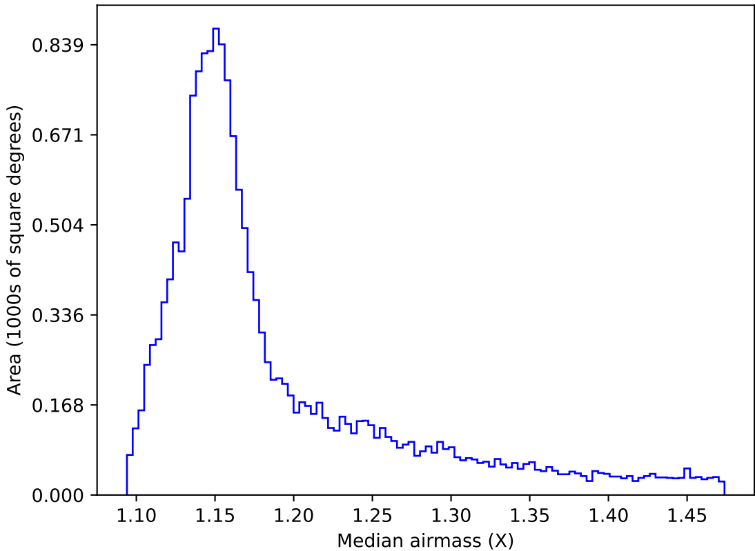
too_elab_r64_d2_giz_v3.4_10yrs WFD y band: Median airmass
