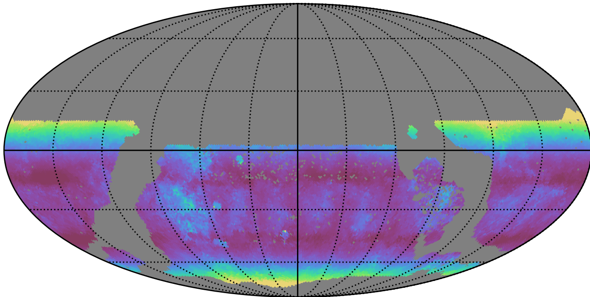
too_elab_r64_d2_giz_v3.4_10yrs WFD u band: Median airmass
