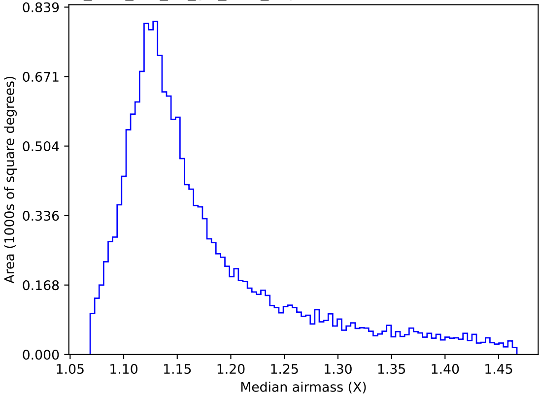
too_elab_r64_d2_giz_v3.4_10yrs WFD u band: Median airmass
