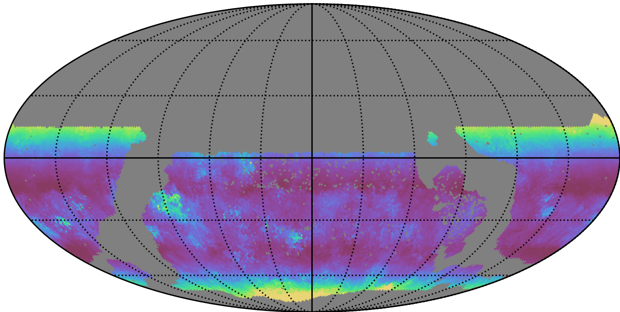
too_elab_r64_d2_giz_v3.4_10yrs WFD g band: Median airmass
