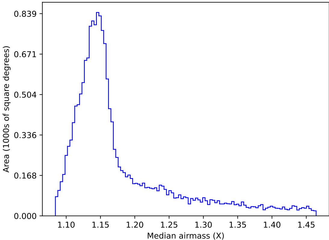
too_elab_r64_d2_giz_v3.4_10yrs WFD all bands: Median airmass
