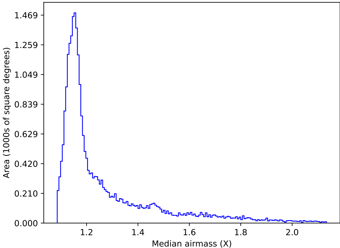
too_elab_r64_d2_giz_v3.4_10yrs All sky z band: Median airmass
