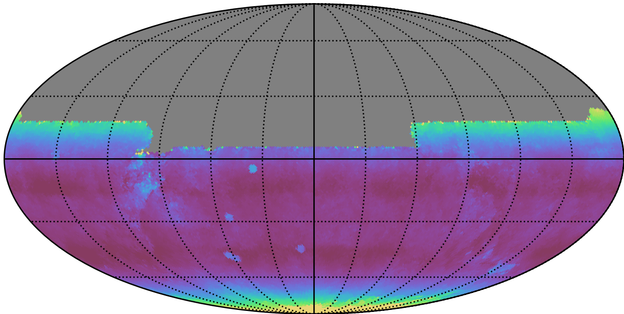
too_elab_r64_d2_giz_v3.4_10yrs All sky y band: Median airmass
